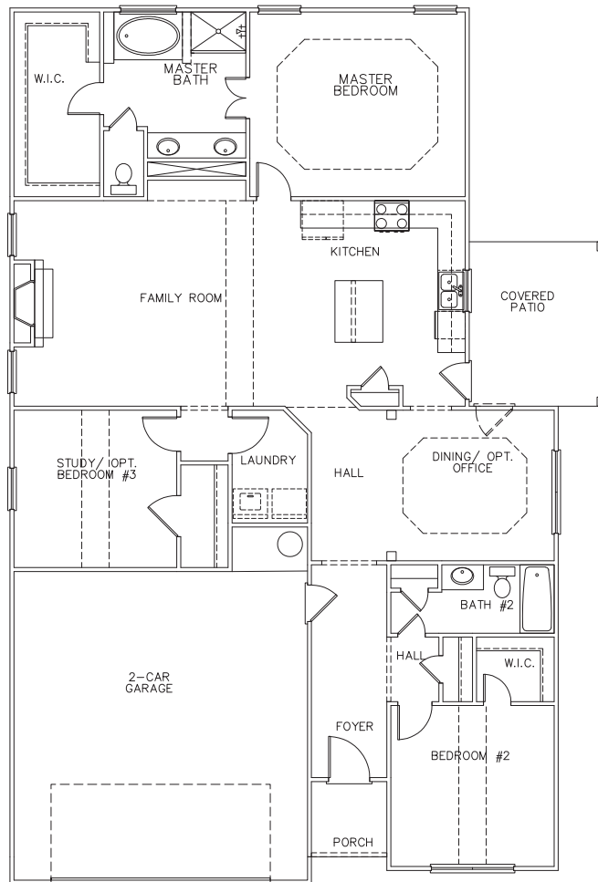
Ranch Plan
